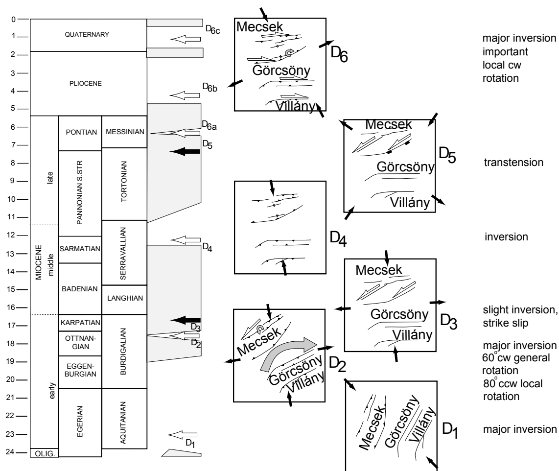
Fig. 11. Synthetic table of structural events. White arrows indicate onset of major structural events. Boxes show structures active during the different deformation phases in original coordinates. Black arrows indicate inferred shortening and elongation directions. Grey arrows indicate rotations. D 1 –D 6 refer to tectonic events described in the text.
