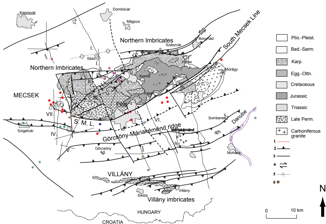
Fig. 4. Structural map of the Mecsek-Villány area based on seismic section reinterpretation (after Wórum 1999, slightly modified). 1 = seismic section network (roman numbers indicate presented sections); 2 = Thrust (dashed: supposed); 3 = Transfer zone; 4 = Strike-slip fault; 5 = Anticline; 6 = Important borehole; S.M.L. = South Mecsek Line; H.L. = Hetvehely Line.
